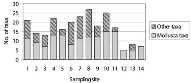
Fig. 2. Total and taxonomic richness of Mollusca at the sampling sites.
