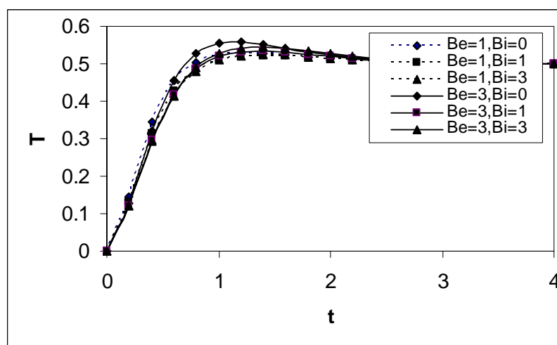
Fig. 2 Effect of the parameters Be and Bi on: (a) u at y=0 ; (b) w at y=0 ; and (c) T at y=0 ( Ha=3 and S=0 )
