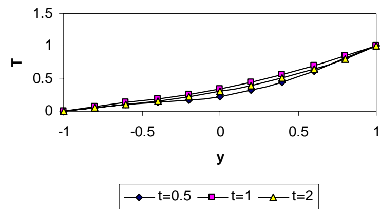
Fig. 1 Time variation of the profile of: (a) u ; (b) w ; and (c) T . ( Ha=3 , Be=3 , Bi=3 , and S=1 ).
