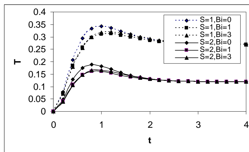
Fig. 4 Effect of the parameters S and Bi on: (a) u at y=0 ; (b) w at y=0 ; and (c) T at y=0 . ( Ha=3 and Be=3 )
