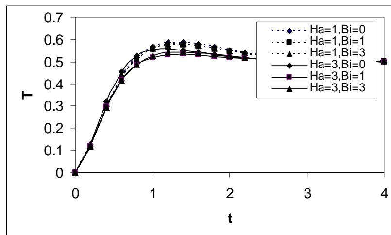
Fig. 3 Effect of the parameters Ha and Bi on: (a) u at y=0 ; (b) w at y=0 ; and (c) T at y=0 . ( Be=3 and S=0 )
